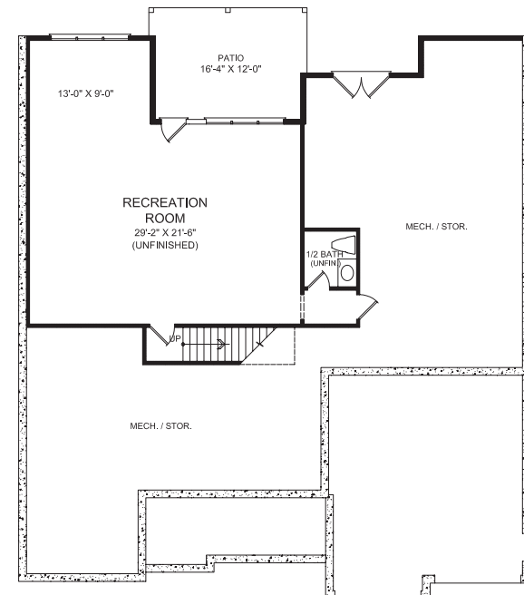
BASEMENT
